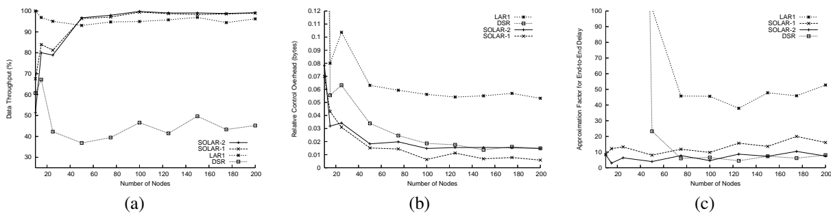
Fig. 7. (a) Data Throughput (b) Relative Control Overhead (c) Approximation Factor for End-to-End Delay, vs. Number of Nodes (Data Connections = 2 \times Number of Nodes)
