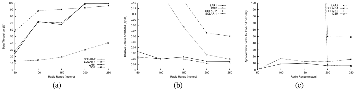
Fig. 6. (a) Data Throughput (b) Relative Control Overhead (c) Approximation Factor for End-to-End Delay, vs. Radio Range (Hub Size = Radio Range)
