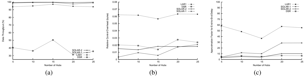
Fig. 3. (a) Data Throughput (b) Relative Control Overhead (c) Approximation Factor for End-to-End Delay, vs. Total hubs
