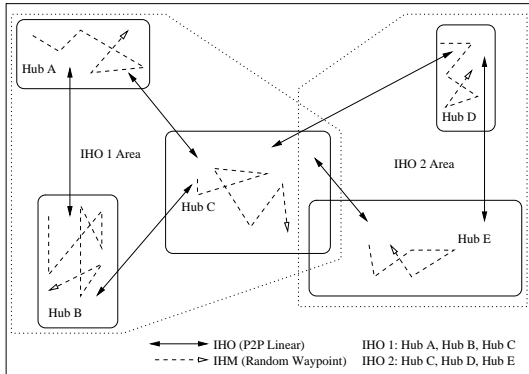
Fig. 2. The random orbit model
