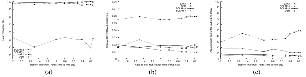
Fig. 5. (a) Data Throughput (b) Relative Control Overhead (c) Approximation Factor for End-to-End Delay, vs. Ratio of Inter-hub Transit Time to Hub Stay Time
