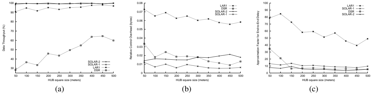
Fig. 4. (a) Data Throughput (b) Relative Control Overhead (c) Approximation Factor for End-to-End Delay, vs. Hub Size
